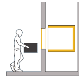
Installation in a restaurant-bar, model 50 kg with wood cladding.
