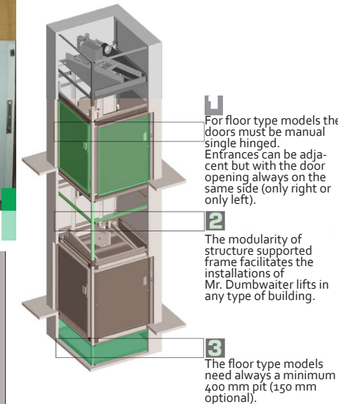
Installation in a commercial airport, model 300kg.
